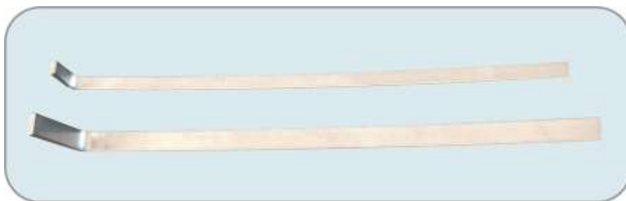
Figure 6-2: Tension wrenches of different sizes
