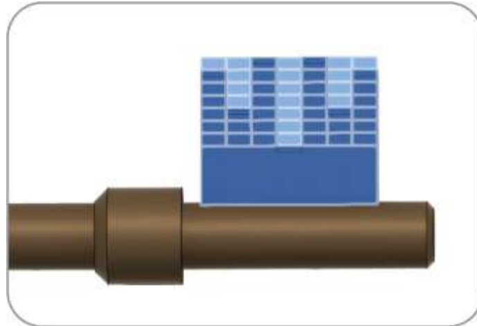
Figure 15-15: Every legal cut on this seven-cut key
