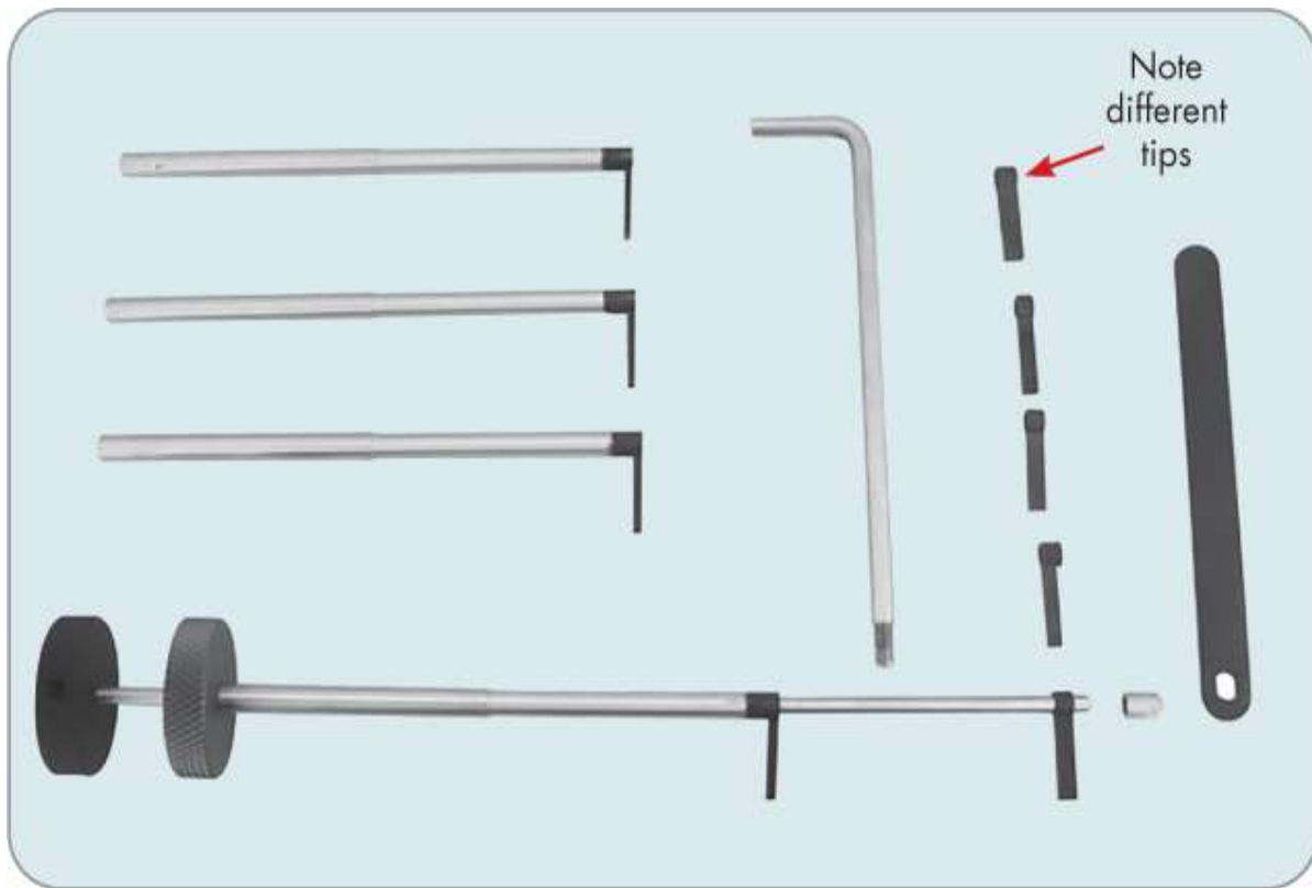
Figure 15-20: Examples of 2-in-1 picks
