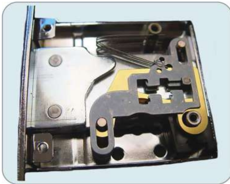
Figure 17-4: The BODA (Finland) 42x double-bitted, eight-lever lock
