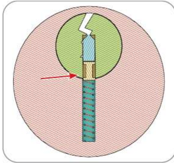
Figure 7-9: A pin stack with a spool pin
