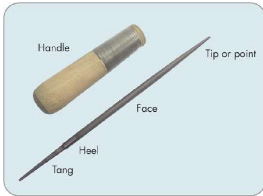
Figure 9-13: Anatomy of a hand file
