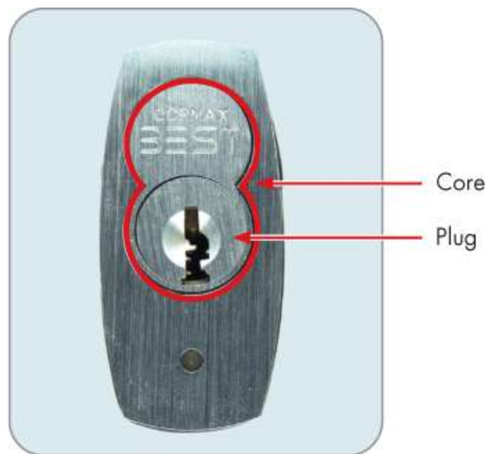
Figure 3-5: An SFIC core in a padlock
