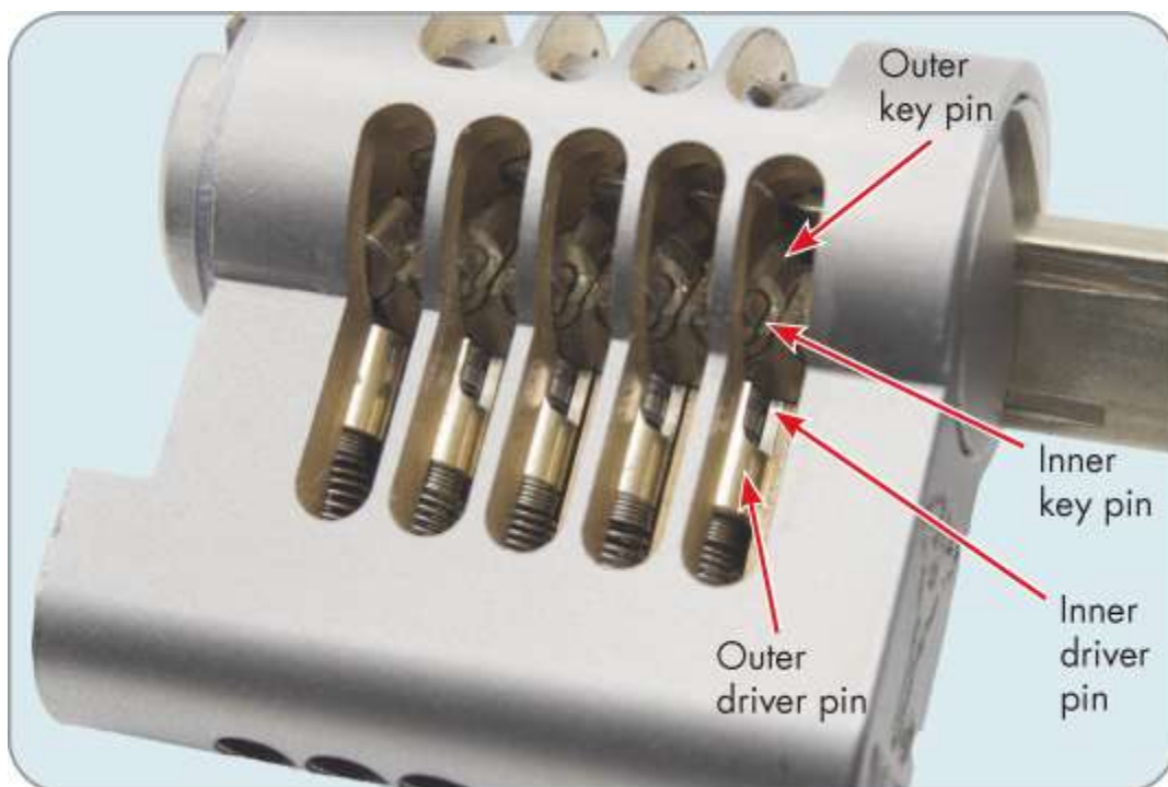
Figure 4-14: A Mul-T-Lock cutaway showing pin-in-pins
