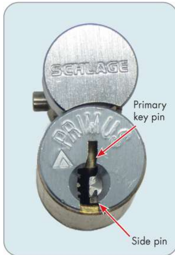
Figure 4-2: A Primus lock with the location of the primary key pin and side pin highlighted
