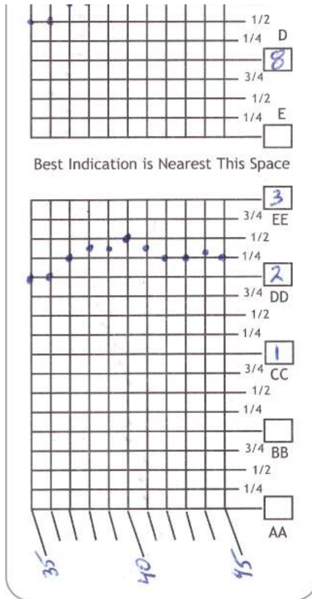
Figure 13-16: Attempting to find True Center after an initial indication of 40
