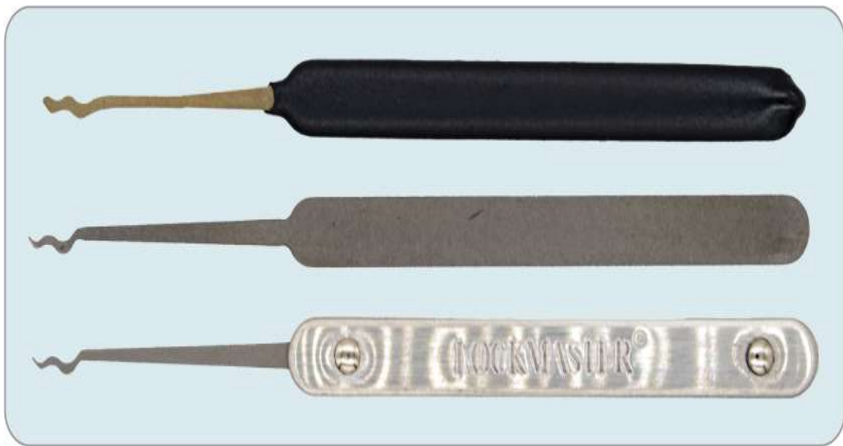
Figure 6-7: Rake handles
