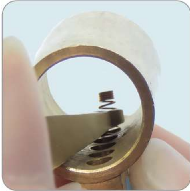
Figure 5-21: Inserting a spring into the bible
