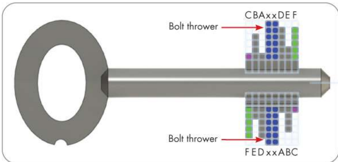
Figure 15-18: The key drives the bolt directly off the two central bits rather than off the opposite side of the key. The "top" bitting pattern is CBAxxDEF, and the "bottom" bitting pattern is the reverse, FEDxxABC.
