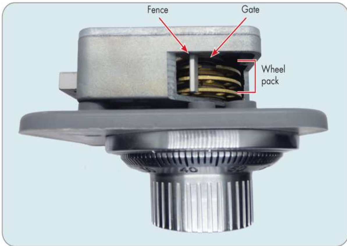
Figure 3-28: A safe lock cutaway showing the wheel pack and fence
