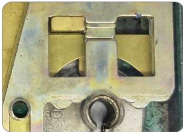
Figure 16-9: Detail of the levers, with the spacers removed and arranged to show the various belly radii as well as possible
