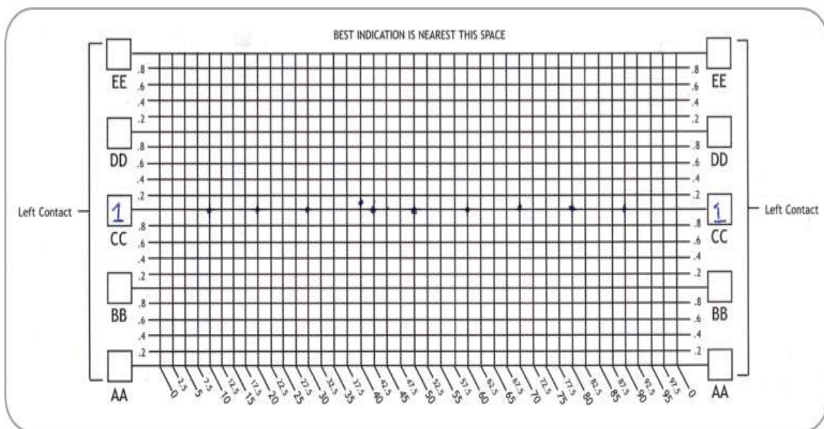
Figure 13-10: Testing the left contact points in increments of 10
