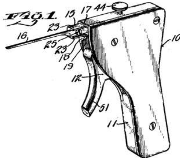
Figure 1-1: Patent 2,309,677 for a "Lock Picking Gun"
