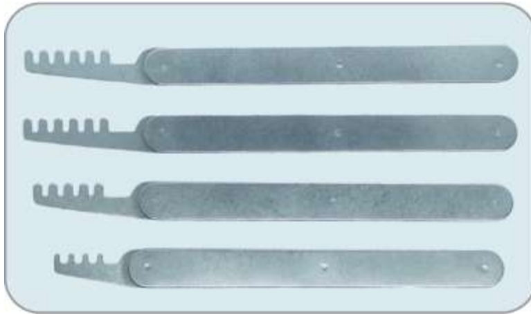
Figure 6-20: A set of comb picks
