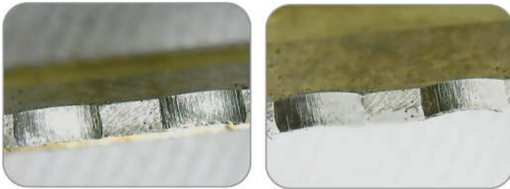
Figure 10-26: The Schlage key surface filed to 11111
