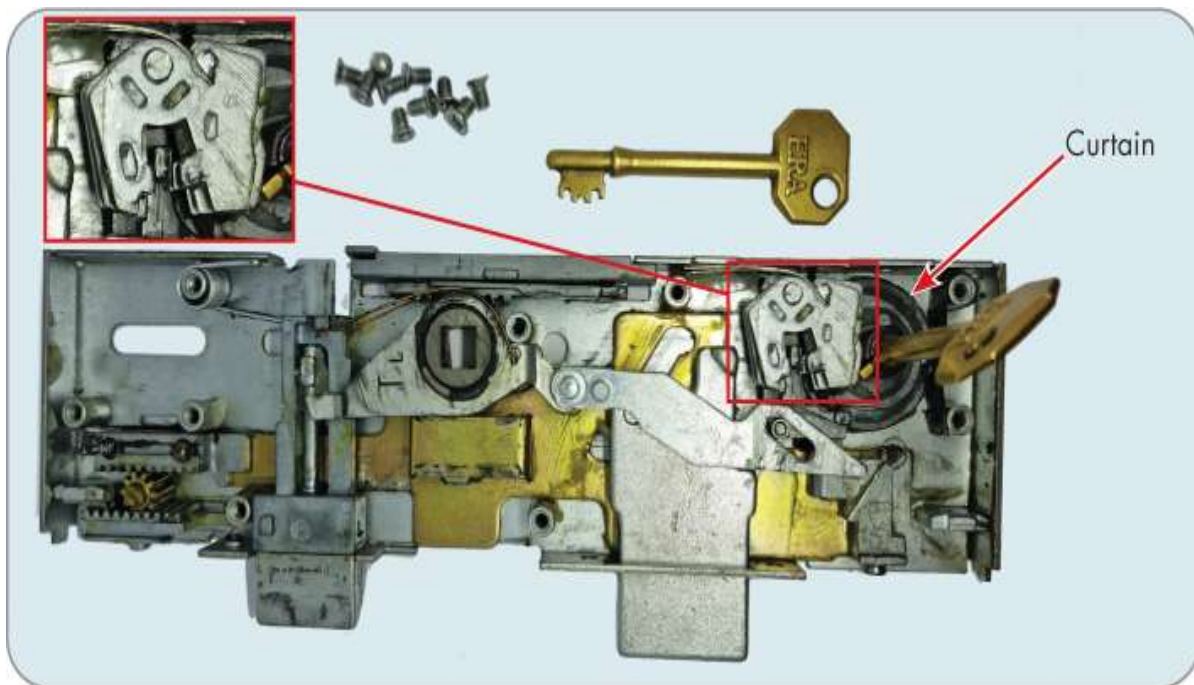
Figure 15-11: In this ERA Vectis multipoint lever lock gearbox, the key is partly turned in the curtain, and the stump has mostly cleared the aligned gates of the lever pack. Unusually for
