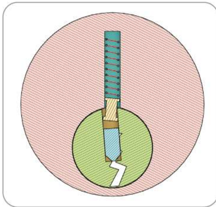
Figure 4-7: A spool pin in a false set
