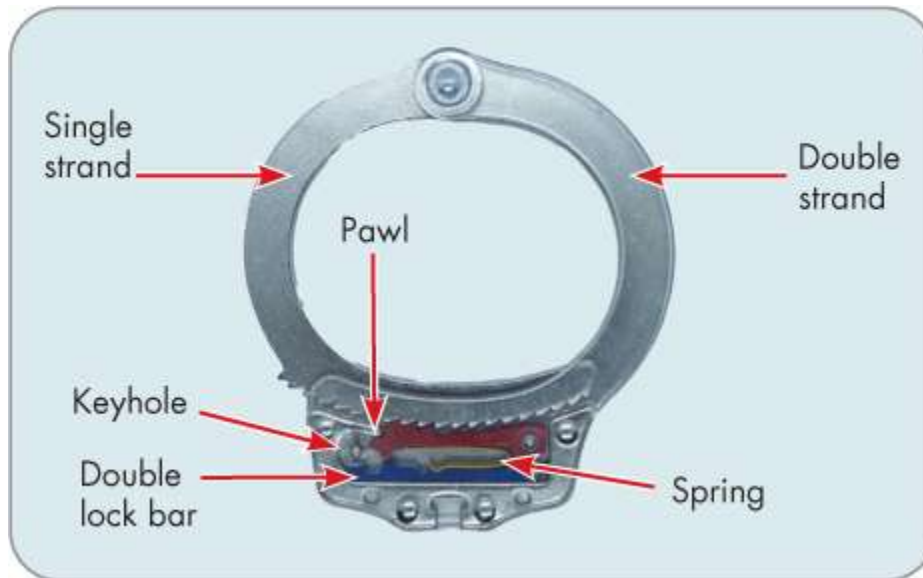
Figure A-12: Cutaway of a standard handcuff
