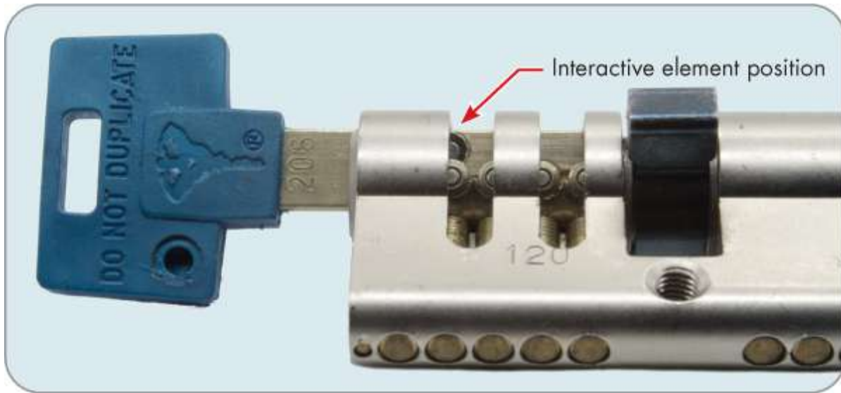
Figure 7-20: Mul-T-Lock Interactive
