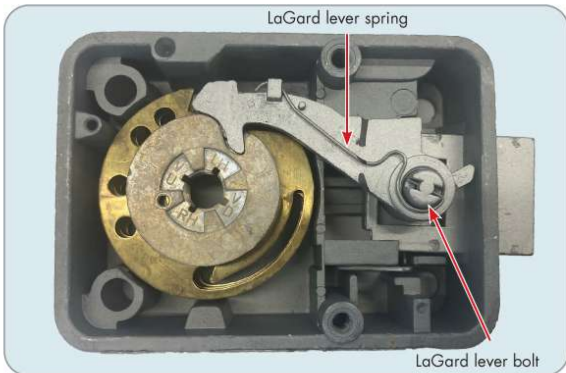
Figure 12-14: The LaGard lever attachment differs from that of other manufacturers.
