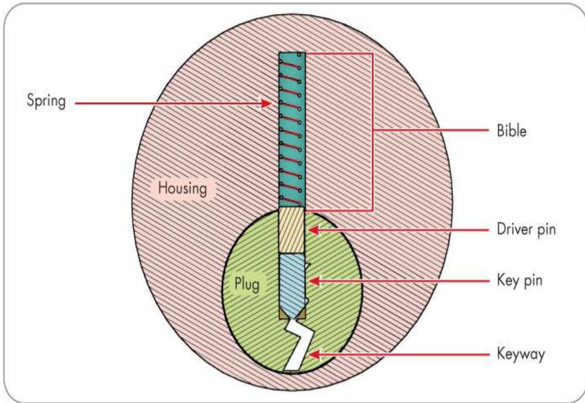
Figure 3-15: The pin stack
