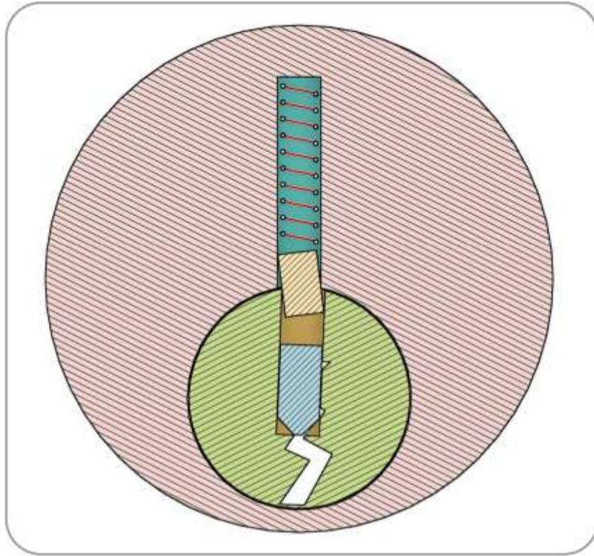
Figure 3-18: A driver pin blocking the plug's rotation
