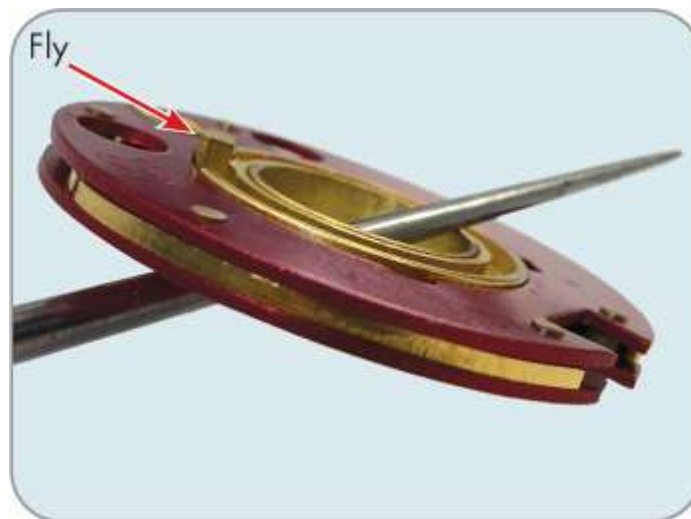
Figure 12-17: Wheel 3, the one closest to the drive cam, always has a protruding fly, while all the other flies are flush with the wheel.
