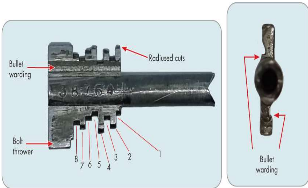
Figure 15-13: A Rosengrens ABN changeable safe-lock key
