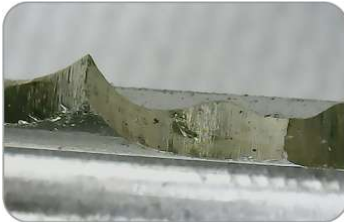
Figure 10-19: An off-center scuff mark
