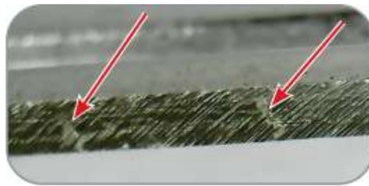
Figure 10-3: Finding spacings by using the polishing technique
