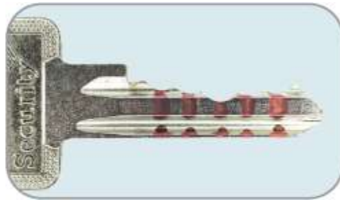
Figure 10-4: A half-cut key with spacing help lines still visible
