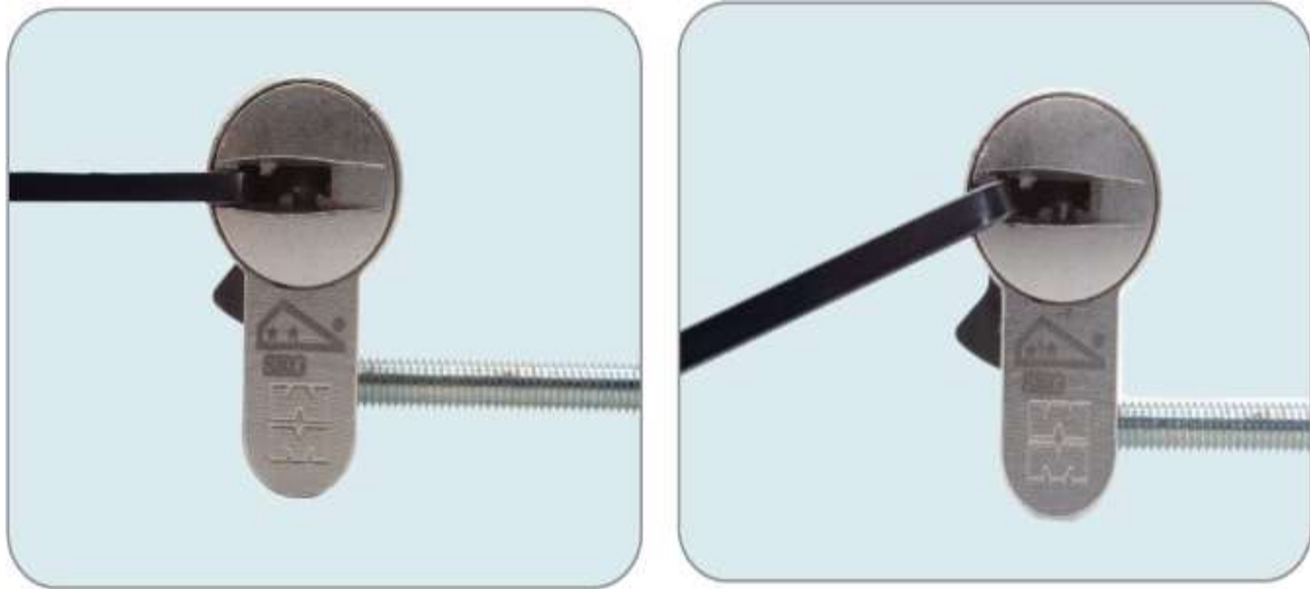
Figure 7-14: Two different sizes of tension wrenches
