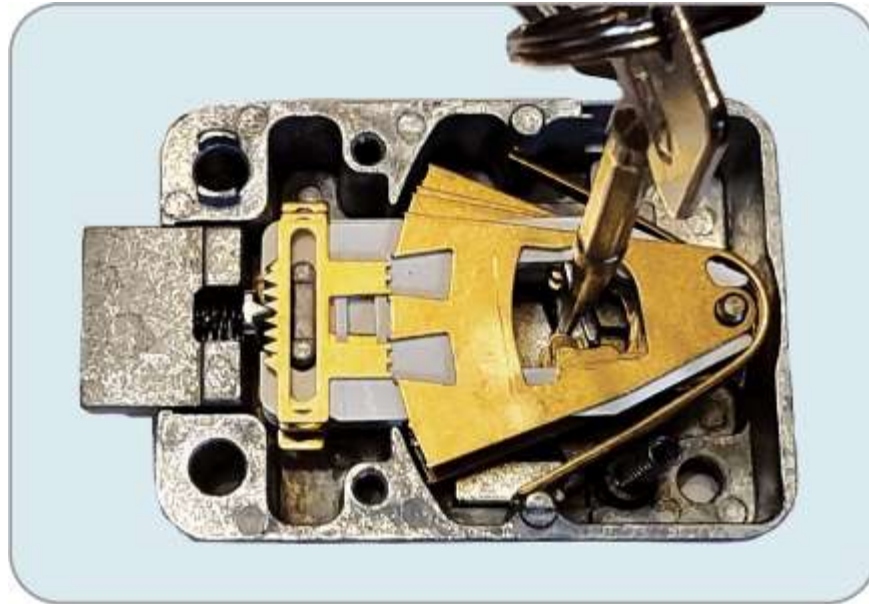
Figure 15-10: A high-end safe lock, the S&G/FAS 6890
