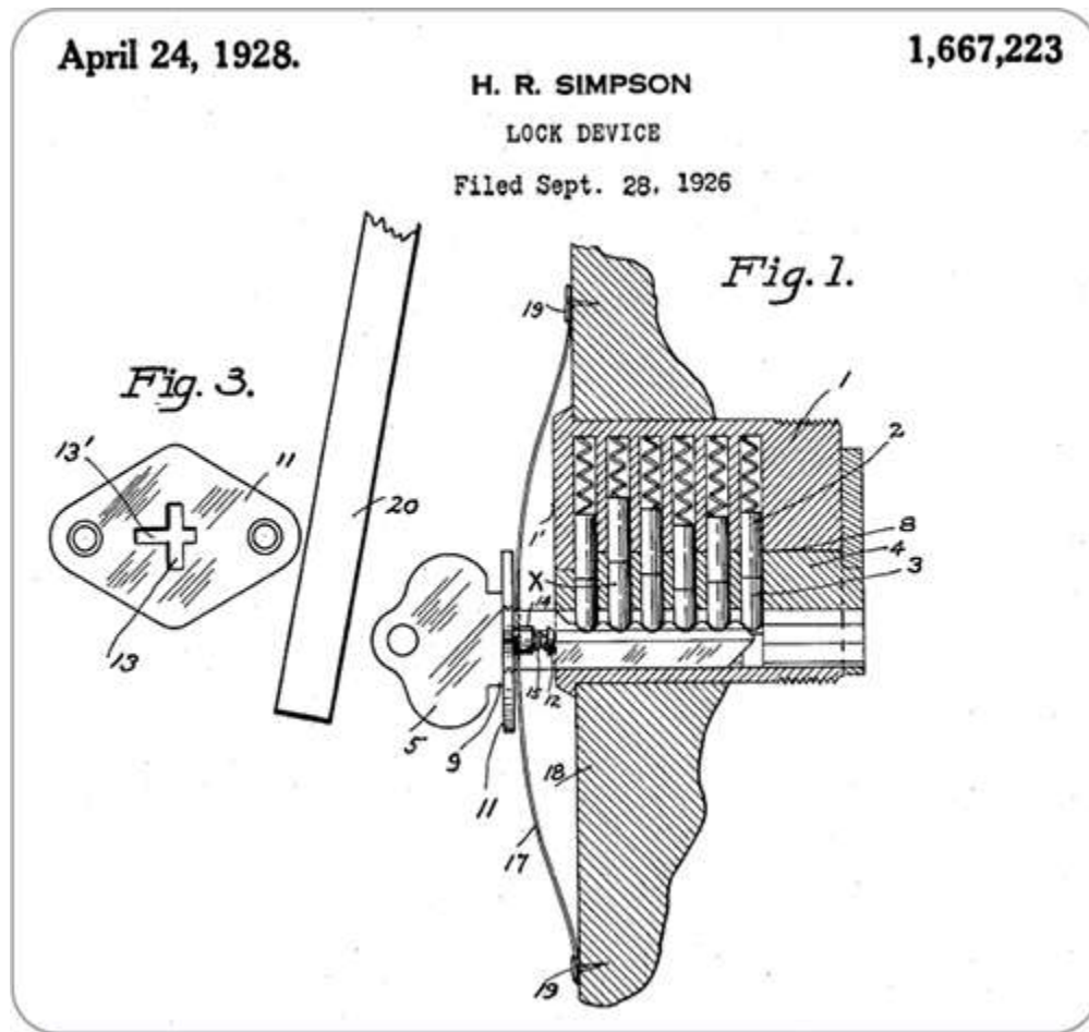
Figure 1-2: Patent 1,667,223 for a "Lock Device"
