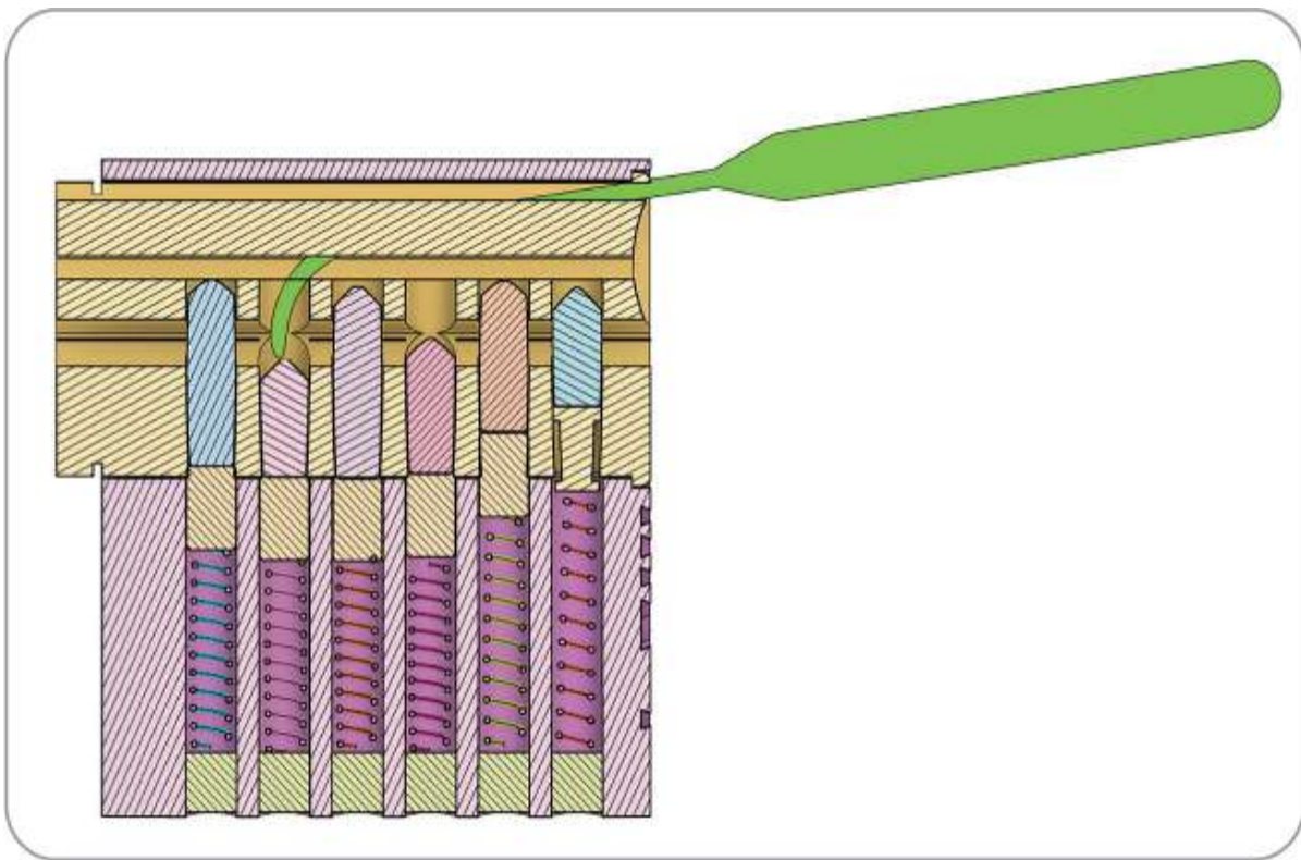
Figure 6-12: A gonzo hook being used to move a short key pin
