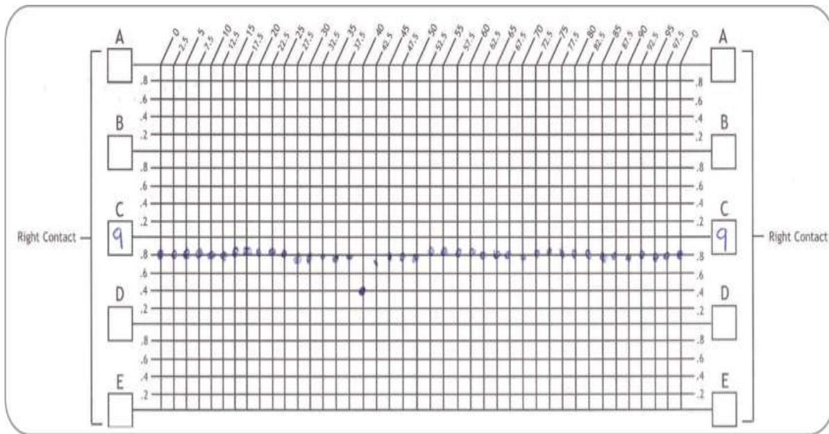
Figure 13-9: The right contact point has little movement except in one area of the dial.
