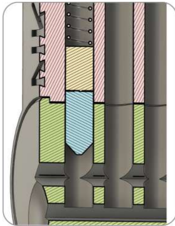
Figure 3-17: A key pin blocking the plug's rotation
