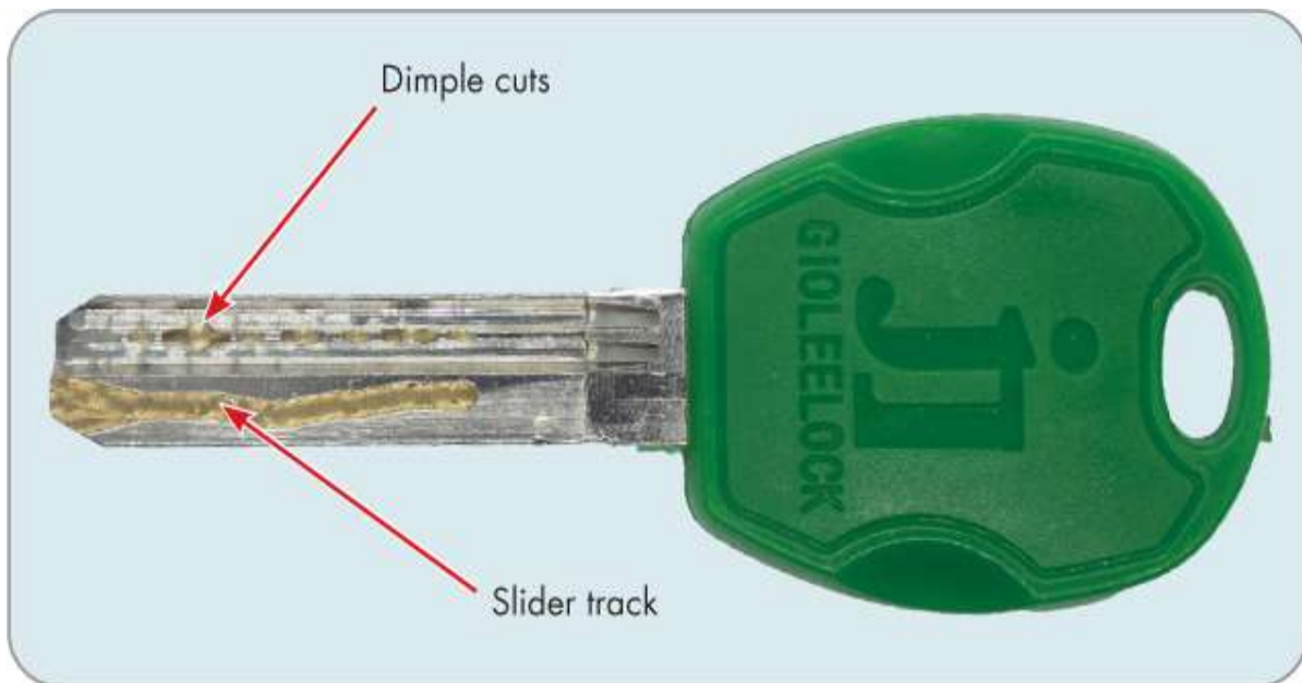
Figure 4-18: A dimple lock key with a slider track
