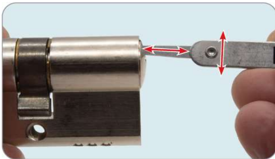
Figure 7-8: The raking movement
