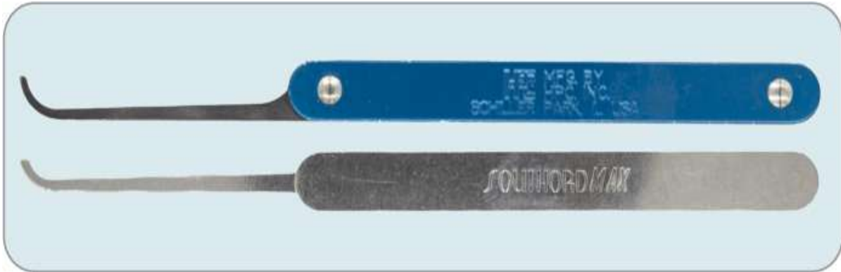
Figure 6-11: A gonzo hook (top) next to a regular hook (bottom)
