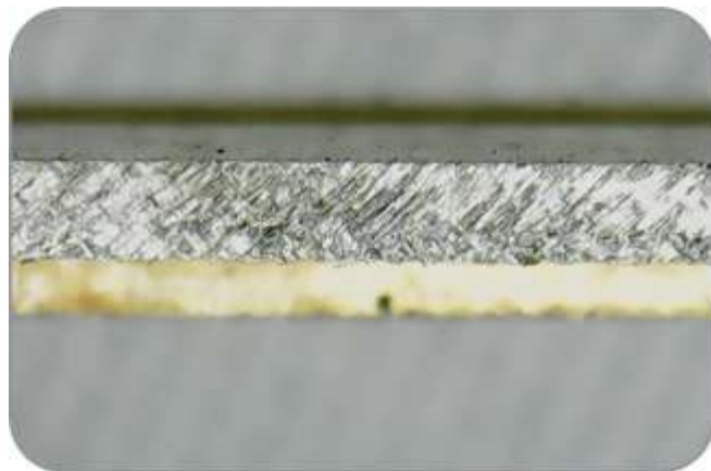
Figure 10-24: The Schlage key with coating removed
