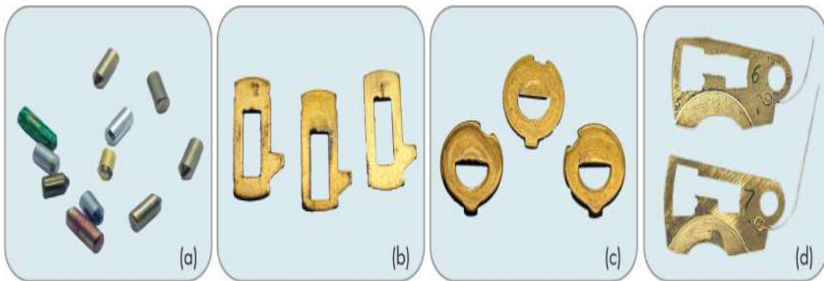
Figure 3-8: An assortment of key and driver pins (a), wafers (b), discs (c), and levers (d)
