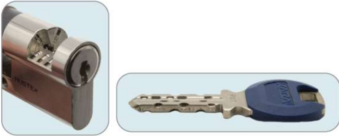
Figure 7-22: Kaba Quattro cylinder and key
