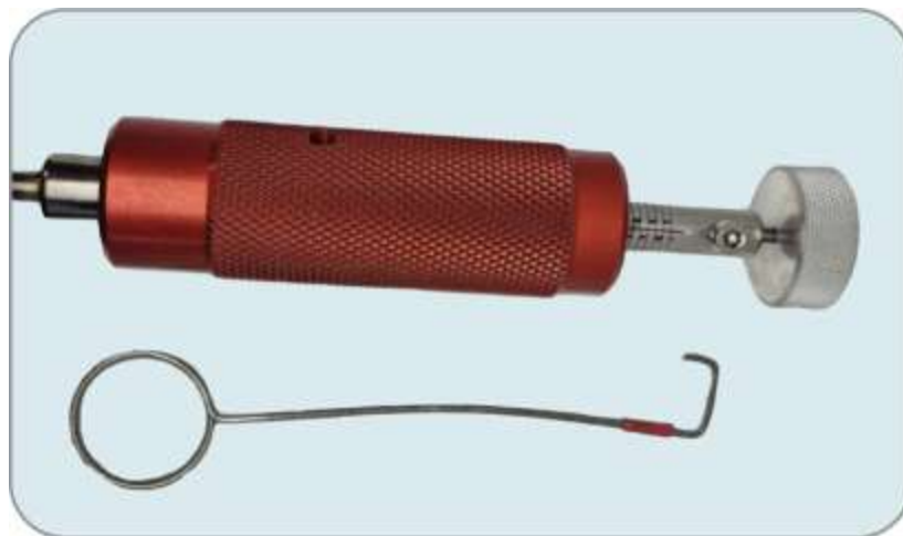
Figure 15-23: Both of these tools started off straight: the handle to a custom-made pick for the Mauer 71111 President lock, complete with engraved spacing markings for each lever, by Jason Jones at https://www.kelocks.co.uk (top), and a J wire (bottom).
