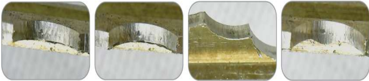
Figure 10-32: Various Schlage marks
