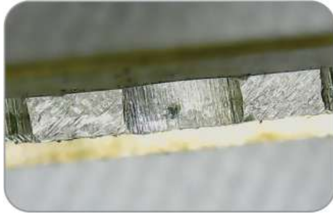
Figure 10-27: First (faint) mark on the Schlage key
