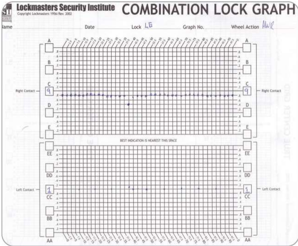
Figure 12-9: This Lockmasters chart breaks the increments into fifths.
