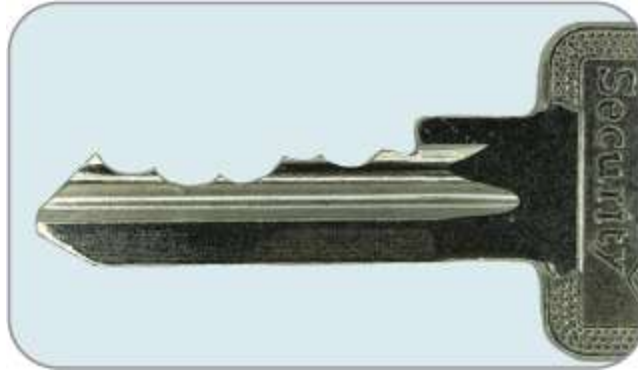
Figure 10-22: An impressioned C83 key
