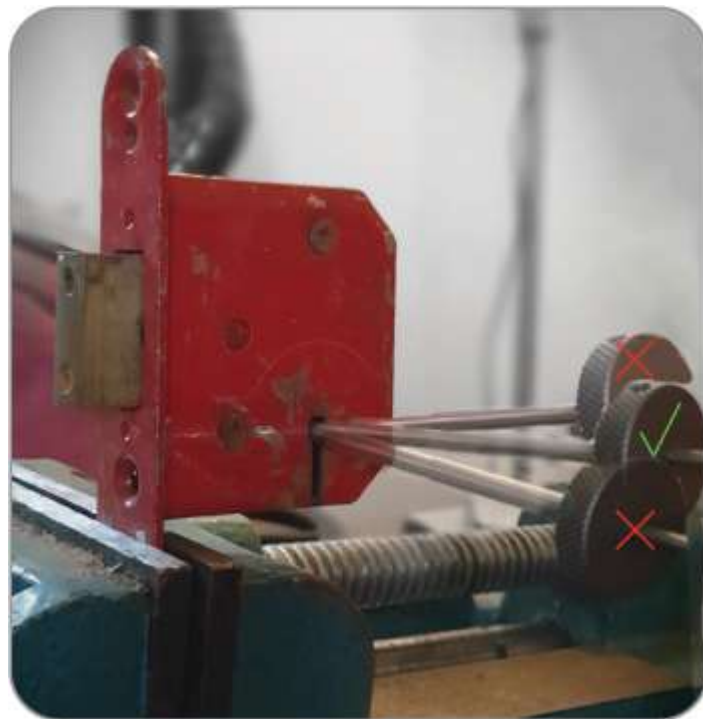
Figure 17-7: Keep your picking tool square to the lock face. If you compress the pack, take care to pull the tensioner straight outward, not tilting it, as the picking arm will hit multiple levers if you do.
