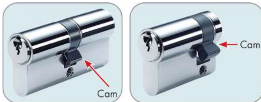
Figure 7-5: Euro profile cylinders
