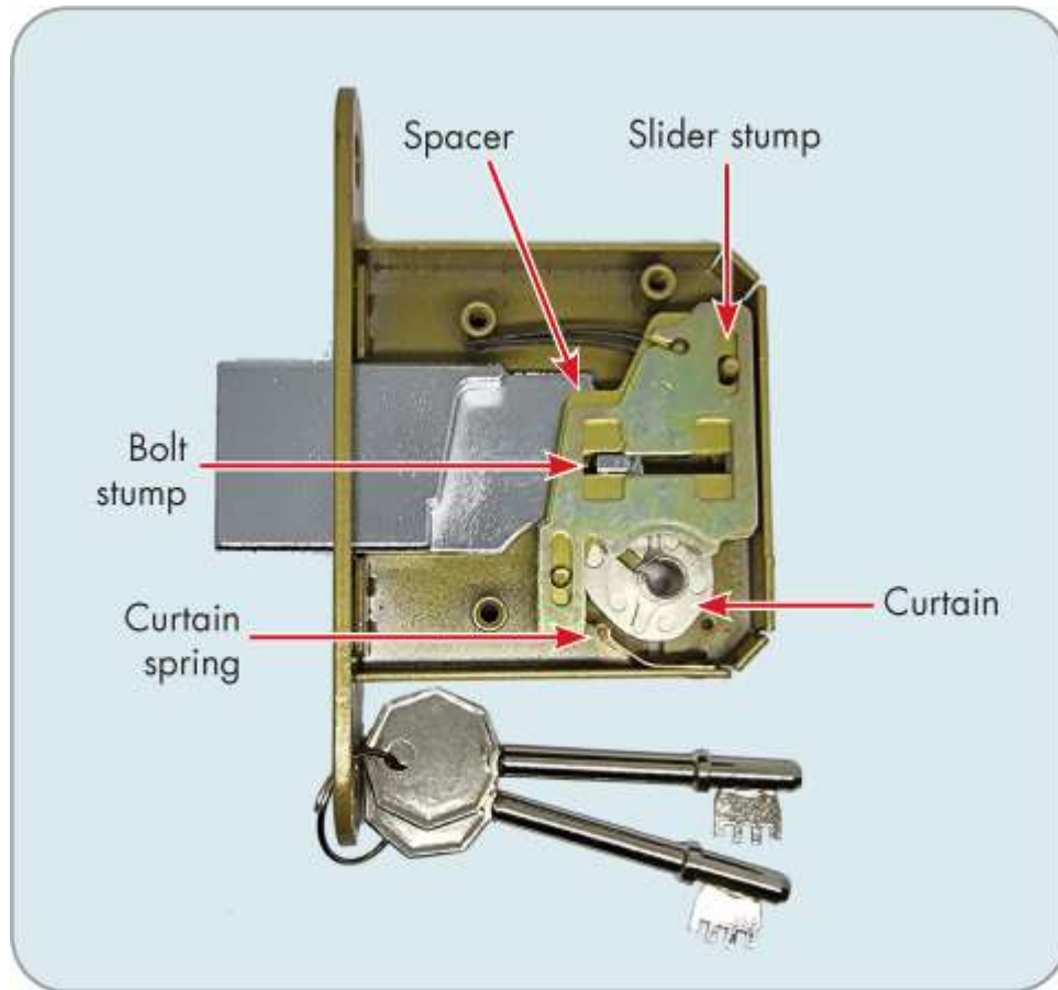
Figure 15-9: An Asec British Standard five-lever deadlock
